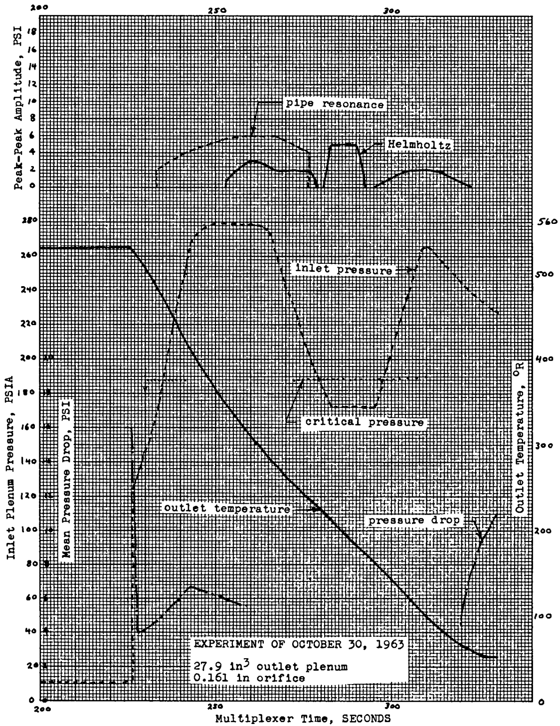
Figure 42. Pressures, Temperatures, Amplitudes - October 30, 1963
