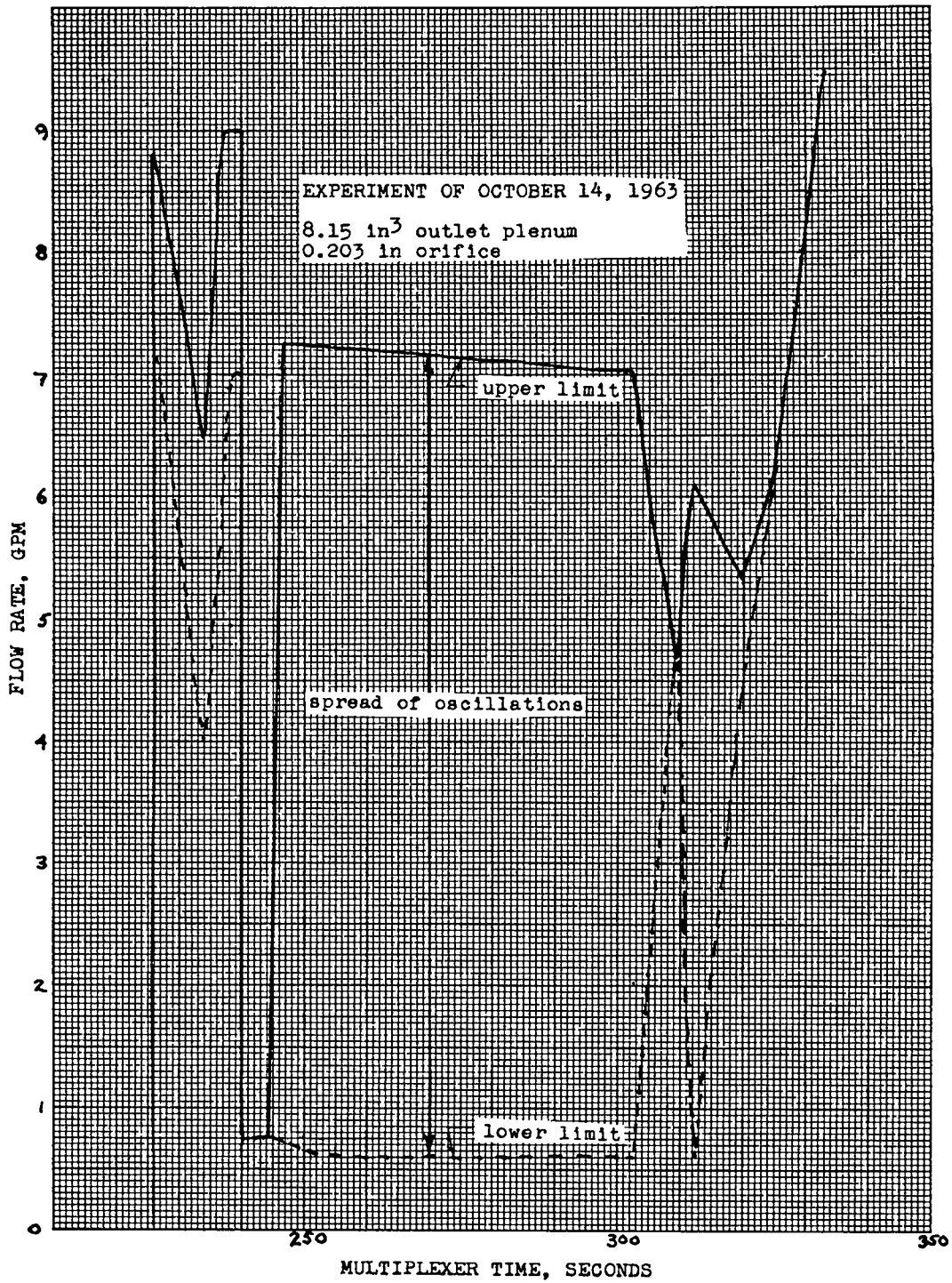
Figure 20. Flow Rate - October 14, 1963
